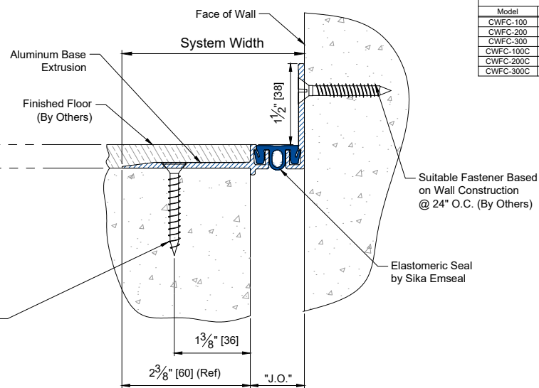
CWFC [100C] DECK TO WALL CONDITION
