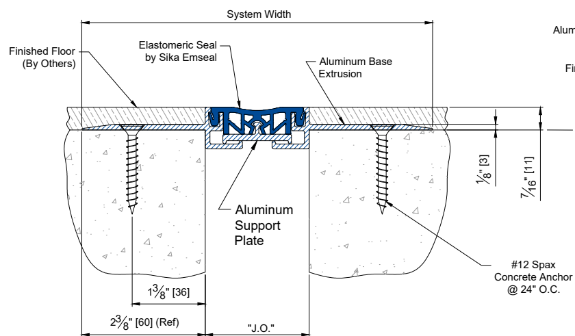
CWFC [200-300] DECK TO DECK CONDITION
