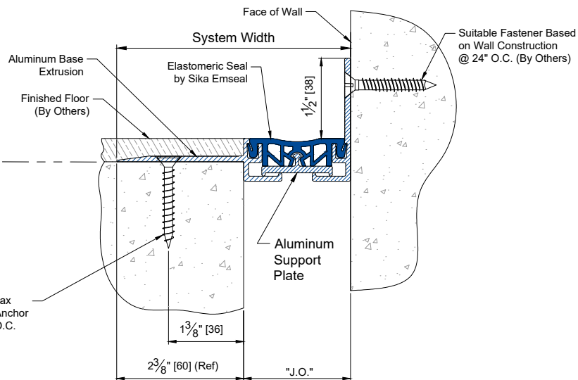
CWFC [200C-300C] DECK TO WALL CONDITION
