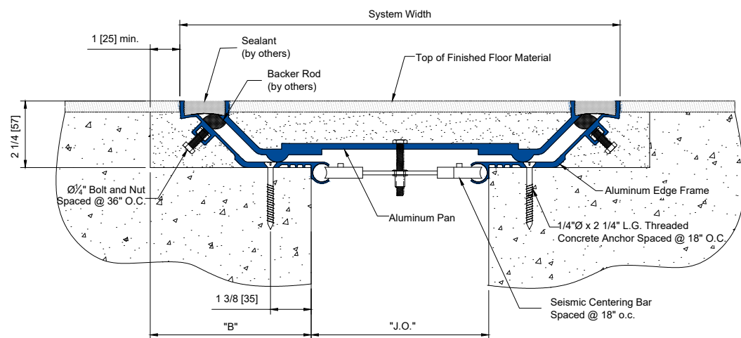
SPJ [400-1800] DECK TO DECK CONDITION
