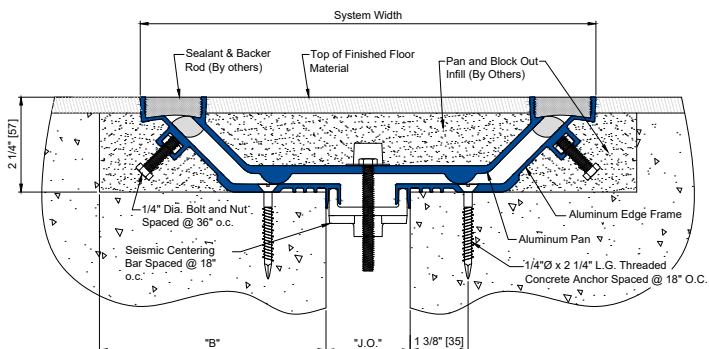
SPJ [200] DECK TO DECK CONDITION
