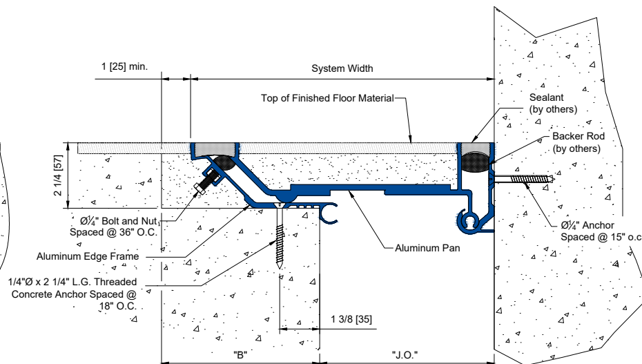
SPJ [400C-1800C] DECK TO WALL CONDITION
