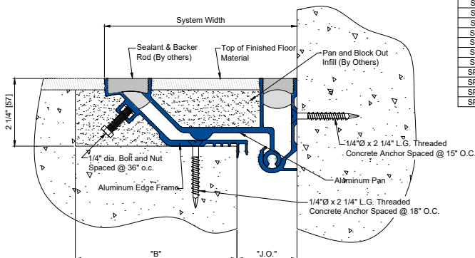
SPJ [200C] DECK TO WALL CONDITION
