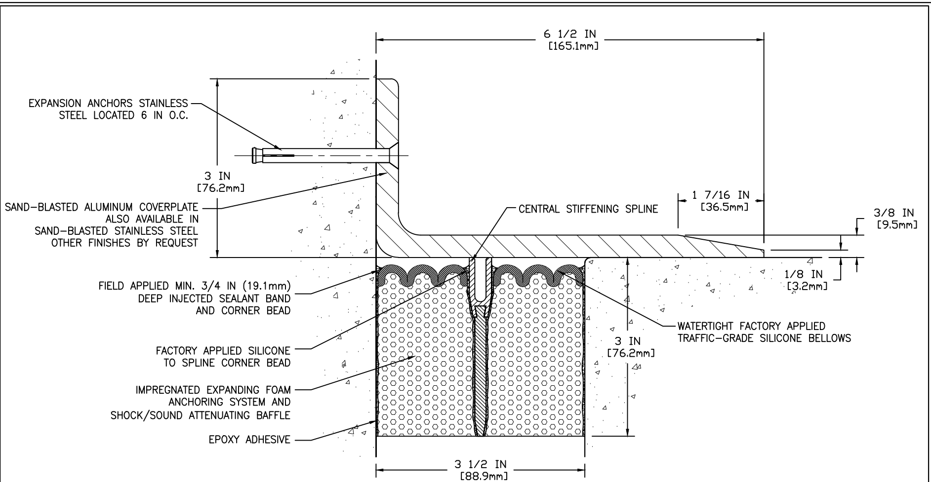
CROSS SECTION SJS-M-0350-CVRX-M-38-06.50-DW-LC-SYS
