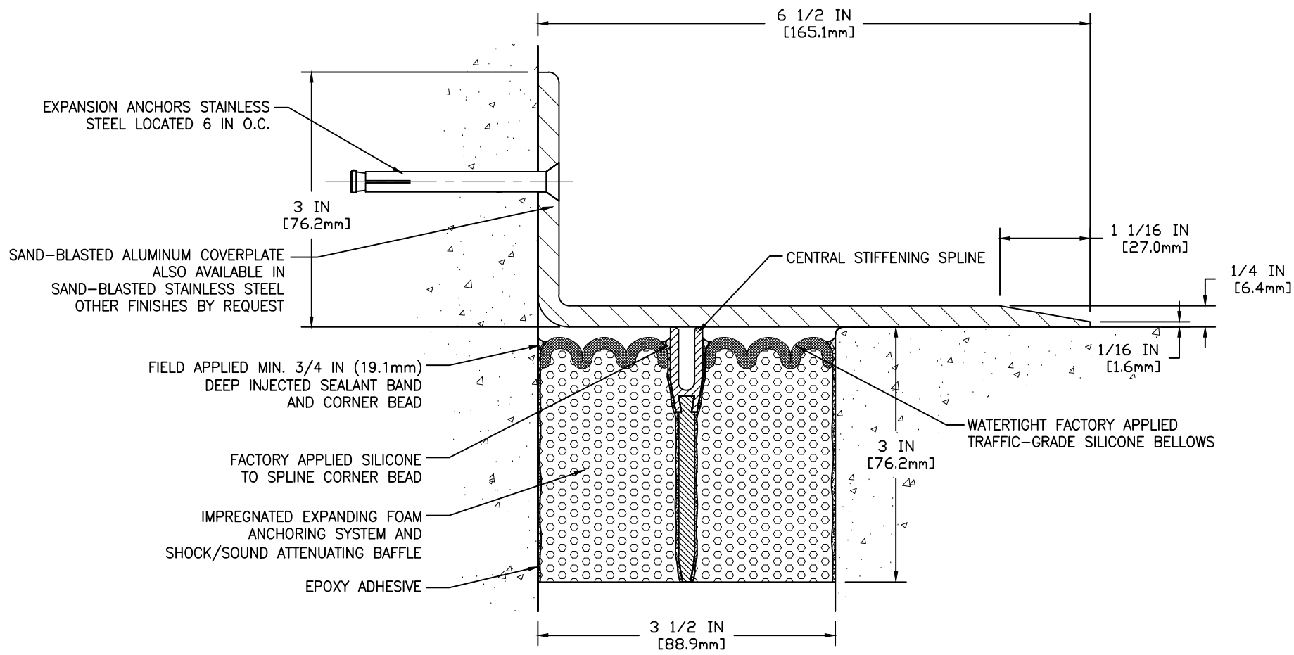
CROSS SECTION SJS-M-0350-CVRX-M-25-06.50-DW-LC-SYS
