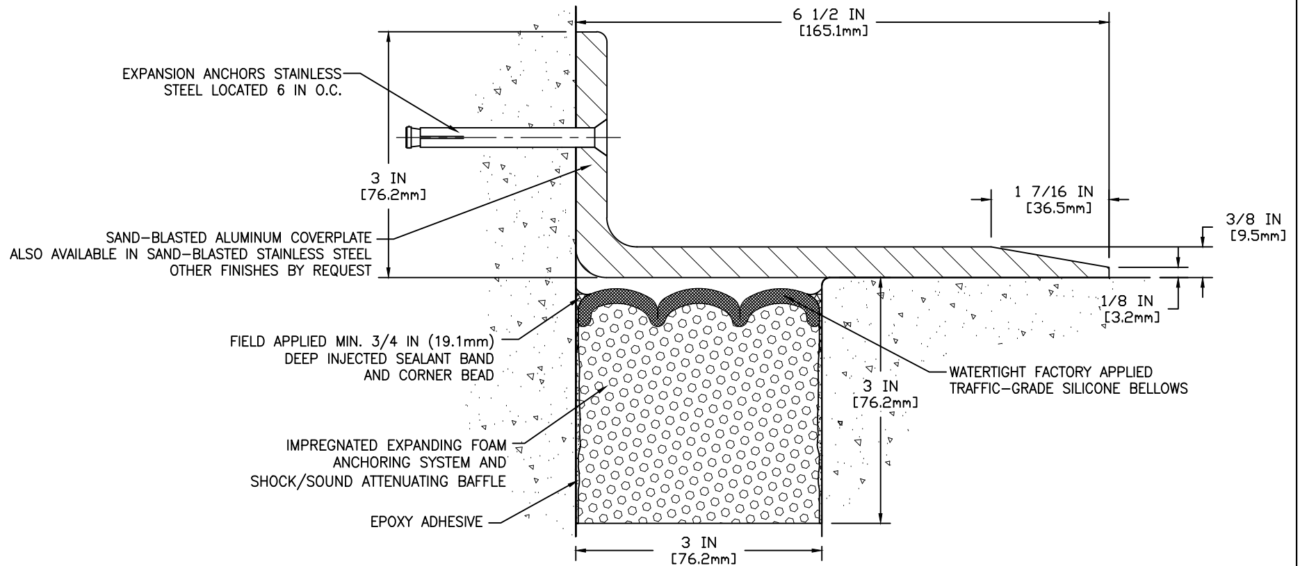
CROSS SECTION SJS-M-0300NS-CVRX-M-38-06.50-DW-LC-SYS
