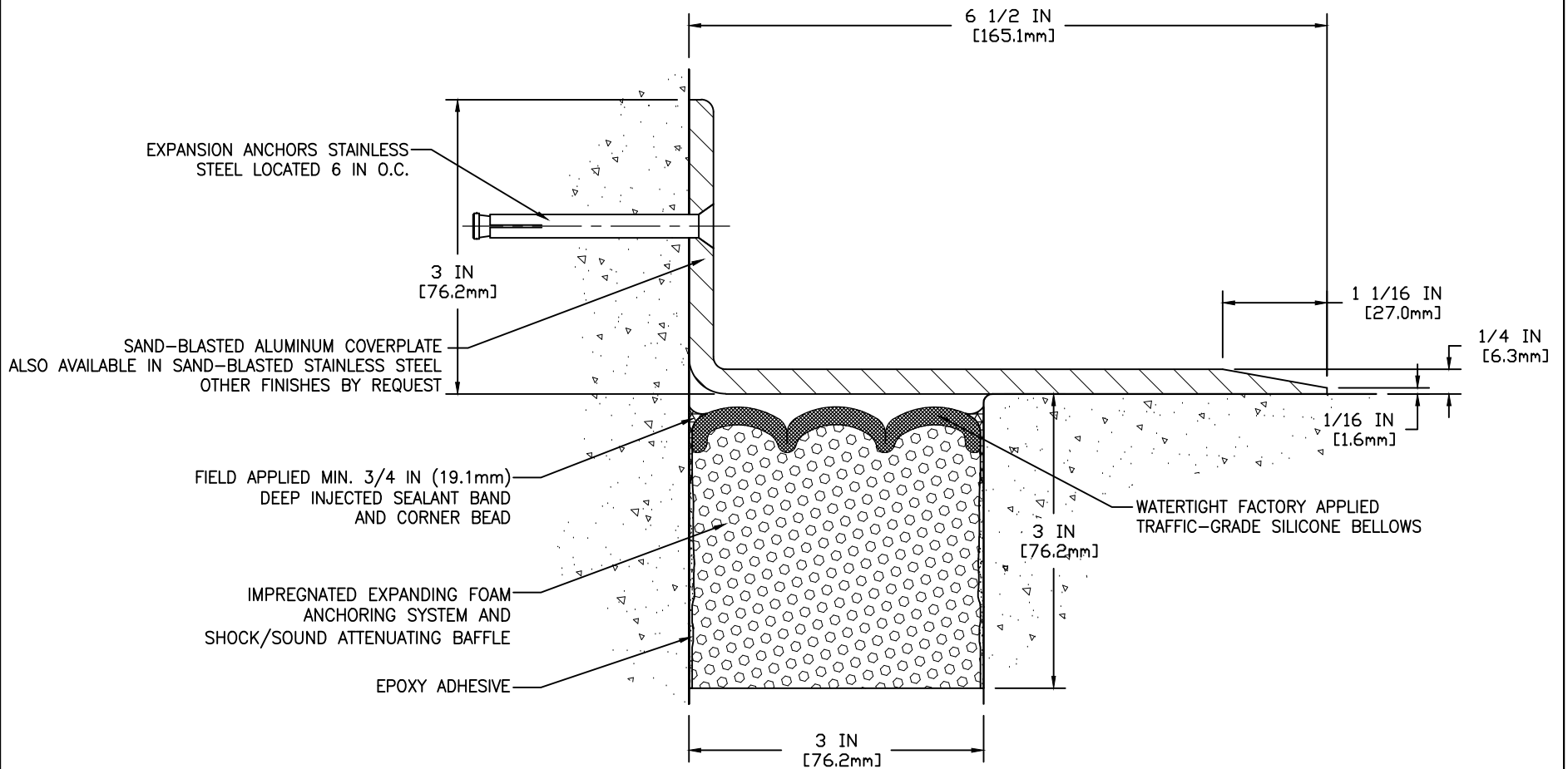
CROSS SECTION SJS-M-0300NS-CVRX-M-25-06.50-DW-LC-SYS
