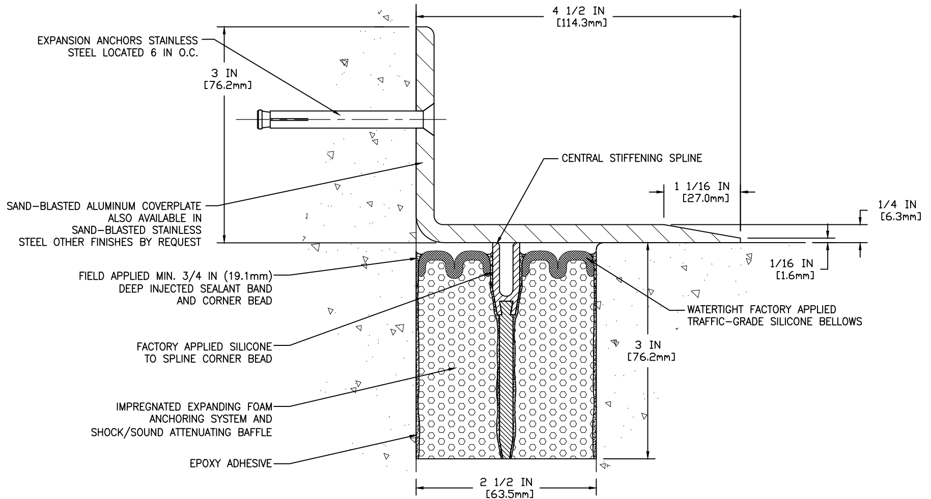
CROSS SECTION SJS-M-0250-CVRX-M-25-04.50-DW-LC-SYS
