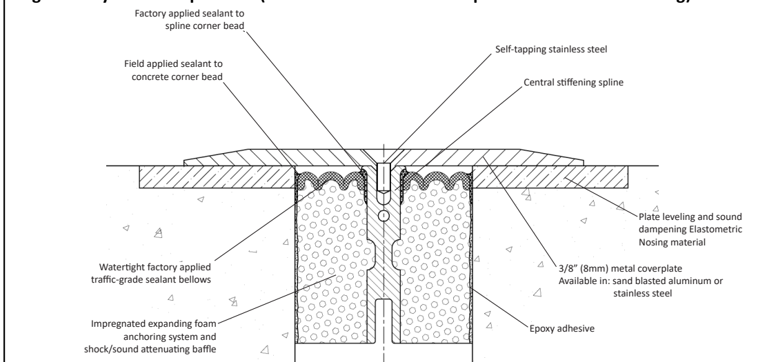
Figure 1: System Components (shown in substrate with optional elastomeric nosing)
