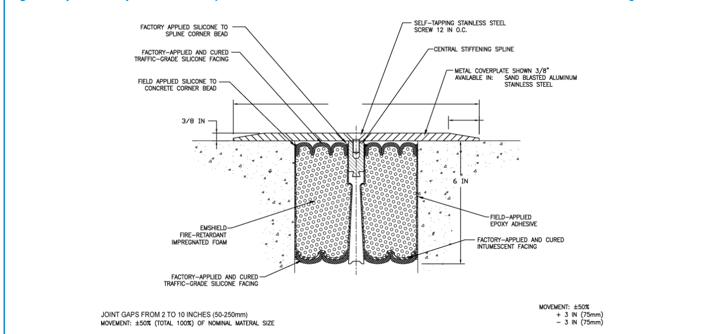
Figure 1: System Components (6-inch system for illustration. Available from 2-inch to 10-inch with Silicone or STPE coating)
