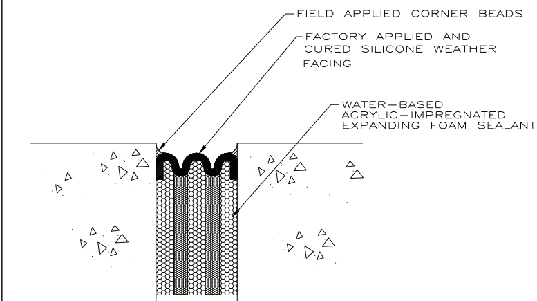
FIGURE 1: COLORSEAL in Typical Installation (substrates may vary).
