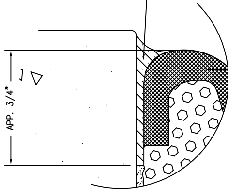
TYPICAL CORNER DETAIL NOT-TO-SCALE
